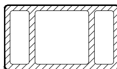
UH38 90 x 51 mm
